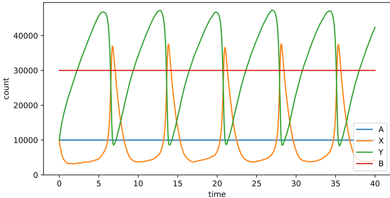
Order-3 Brusselator: rebop, n=10^4
